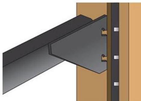
Beds move to three different locations and are secured by a snug steel to steel connection
